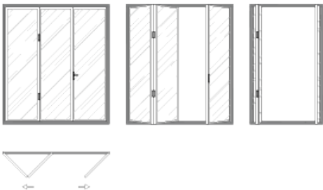
3 Door Series No. of Panel 2+1
