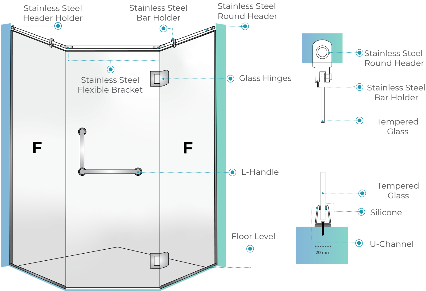
Front View
