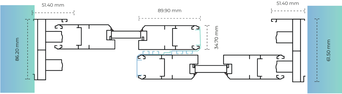
Top View
