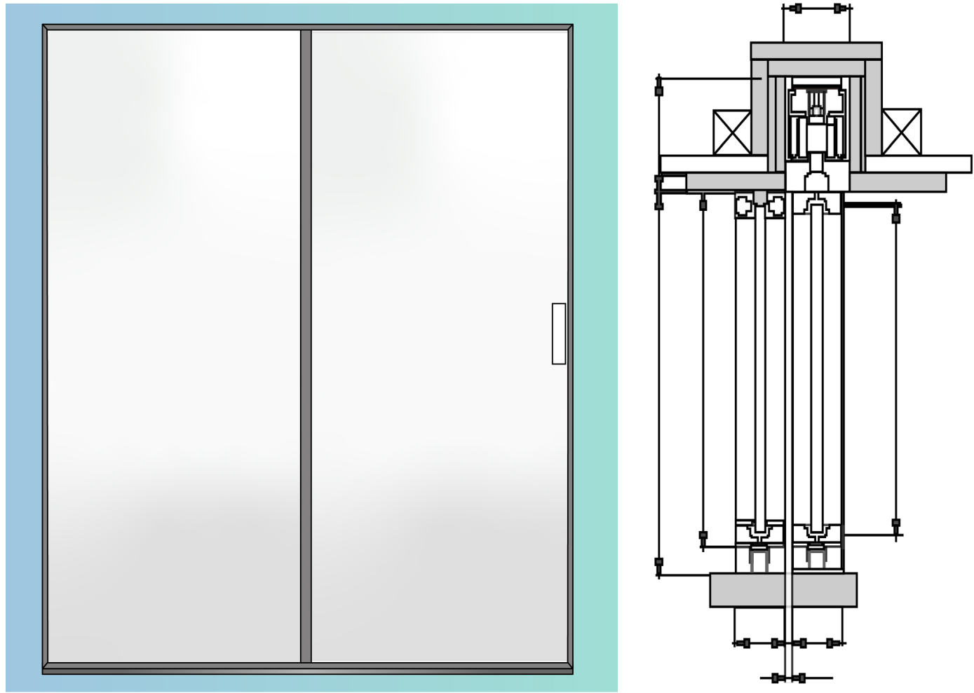
Front View
